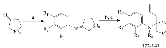
Scheme 6. Preparation of N -(1-allylcycloalkyl)arylamines and their derivatives: (a) \text{ArNH}_2 , benzene or toluene, reflux; (b) allylmagnesium bromide, \text{Et}_2\text{O} , 10–24 °C, then \text{H}_2\text{O} , \text{NH}_4\text{Cl} , ice; (c) \text{Ac}_2\text{O} , \text{Et}_3\text{N} (cat), \Delta ; (d) DDQ, benzene.
