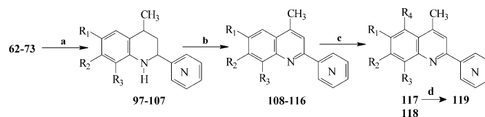
Scheme 4. Transformation of 4-methyl-(tetrahydro)quinolines. (a) \text{H}_2\text{SO}_4 (85%), \text{CHCl}_3 , 90 °C, 10–12 h; (b) S, 270–300 °C, 10–20 min; (c) \text{HNO}_3 , \text{H}_2\text{SO}_4 , –8 °C; (d) \text{NaBH}_4 , Pd/C, MeOH, rt.
