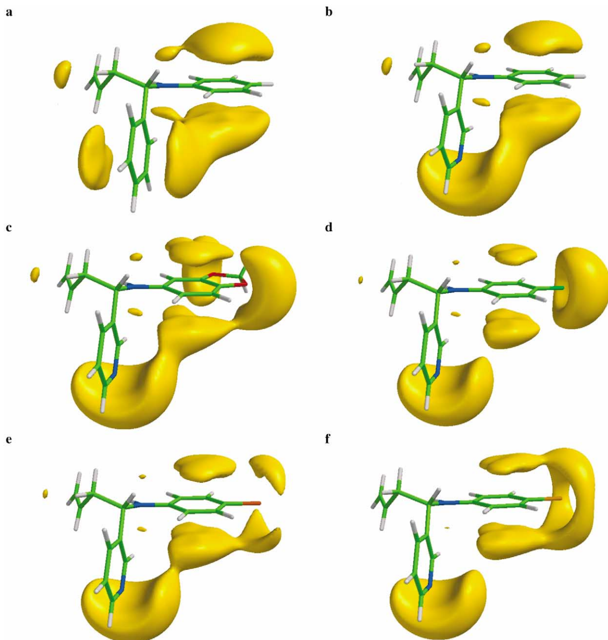
Figure 2. MEPS calculated using the RHF/3-21G optimized geometries for compounds: (a) 53 , (b) 62 , (c) 68 , (d) 69 , (e) 70 , and (f) 71 .
