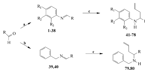
Scheme 1. Preparation of N -substituted aminoalkenes: (a) \text{ArNH}_2 , EtOH (benzene or toluene), reflux; (b) \text{BnNH}_2 , benzene, reflux; (c) allylmagnesium bromide/ \text{Et}_2\text{O} , 10–24 °C, then \text{H}_2\text{O}/\text{NH}_4\text{Cl}/\text{ice} .
