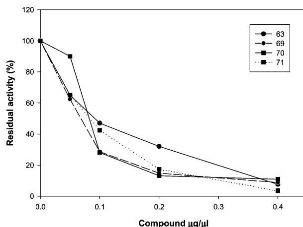
Figure 3. Effect of different concentrations of 4- N -arylamino-4-pyridyl-1-butenes 63 and 69–71 on the in vitro incorporation of [ 14 C]- N -acetylglucosamine into insoluble chitin, expressed as % of residual activity of the enzyme chitin synthase-1.
