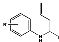
Figure 1. General structure of antifungal homoallylamines.
