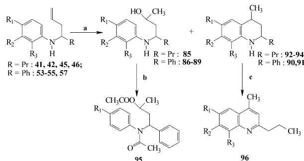
Scheme 3. Transformation of aminoheptenes and aminobutenes: (a) \text{H}_2\text{SO}_4 (75%), 60 °C, 8 h; (b) \text{Ac}_2\text{O} , \text{Et}_3\text{N} (cat), \Delta ; (c) DDQ, benzene.
