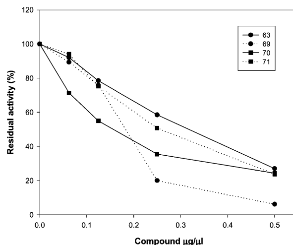
Figure 4. Effect of different concentrations of 4- N -arylamino-4-pyridyl-1-butenes 63 and 69–71 on the in vitro incorporation of [ 14 C]-glucose into insoluble (1,3)- \beta -D-glucan, expressed as % of residual activity of the enzyme (1,3)- \beta -D-glucan synthase.
