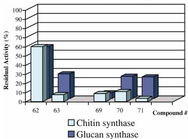
Figure 5. Comparative values of the inhibitory activities of antifungal 4- N -arylamino-4-pyridyl-1-butenes 63 and 69–71 , against (1,3)- \beta -D-glucan synthase and chitin synthase-1, expressed as % of residual activity.
