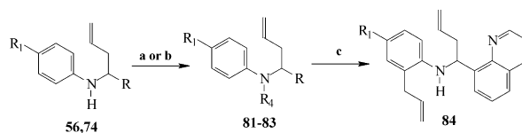
Scheme 2. Transformation of 4- N -arylamino-4-phenyl (8-quinolinyl)-1-butenes: (a) \text{Ac}_2\text{O}/\text{Et}_3\text{N} (cat), \Delta ; (b) allylbromide, \text{K}_2\text{CO}_3 , acetone, reflux; (c) \text{BF}_3\text{Et}_2\text{O} , reflux.
